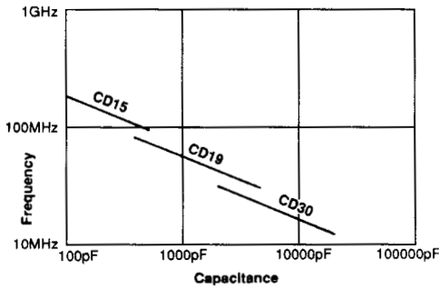
Self-Resonant Frequency
