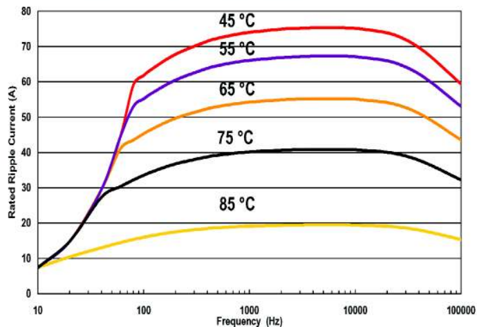
490 \mu\text{F} 800 V Rated Ripple Current, Still Air, 5 kh Life
