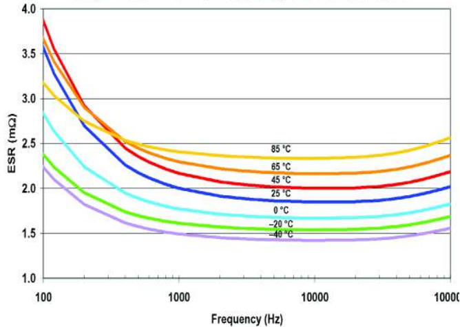
160 \mu\text{F} 1200 V ESR vs Frequency and Temperature
